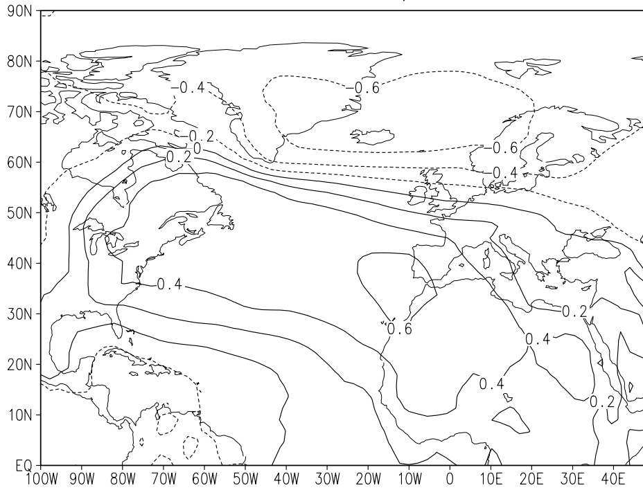
SLP CCA mode of SLP/TA, ERA data
