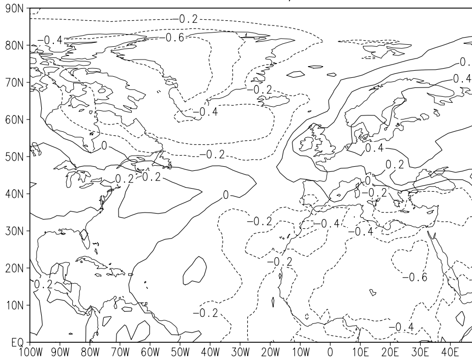
TA CCA mode of SLP/TA, ERA data
